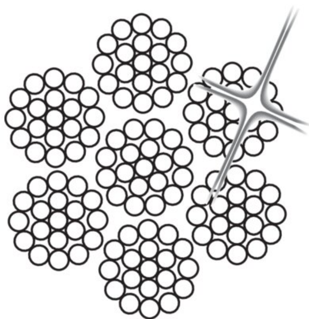
Winch rope
